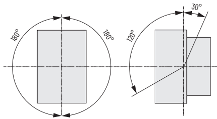
Figure 76 - 100-E116K..., 100-E146K... Contactors
