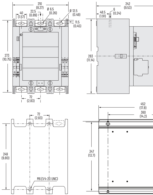
Figure 89 - 100-E580...100-E750 Contactors with PLC Input
