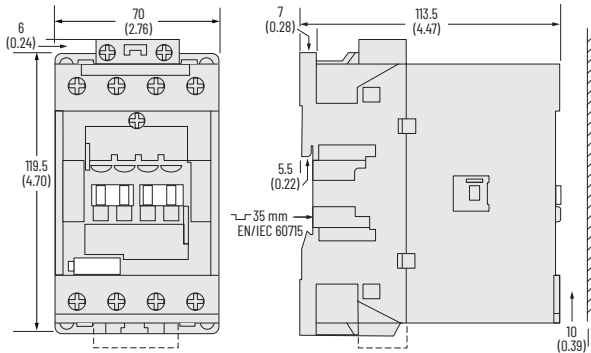
Figure 62 - 100-E40...100-E52 4-Pole Contactors
