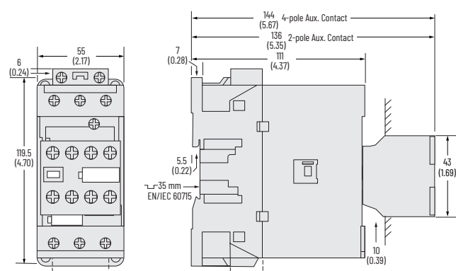
Figure 58 - 100-E40...100-E65 3-Pole Contactors with Front-mounted Auxiliary Contact
