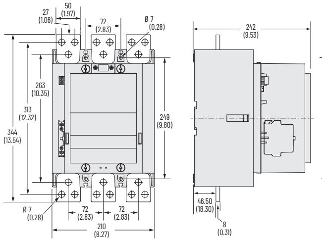
Figure 90 - 100-E1260 Contactors with PLC Input
