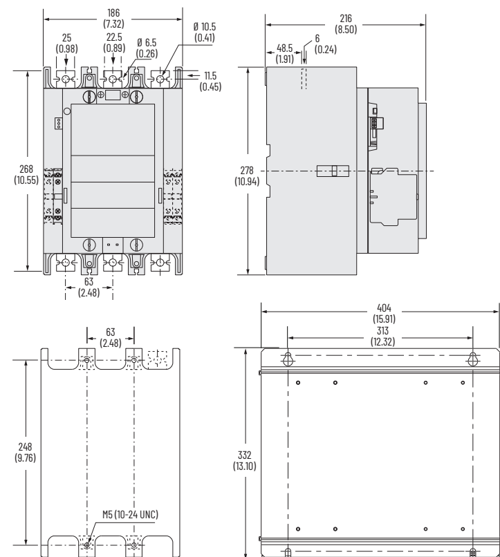
Figure 88 - 100-E400, 100-E460 Contactors with PLC Input
