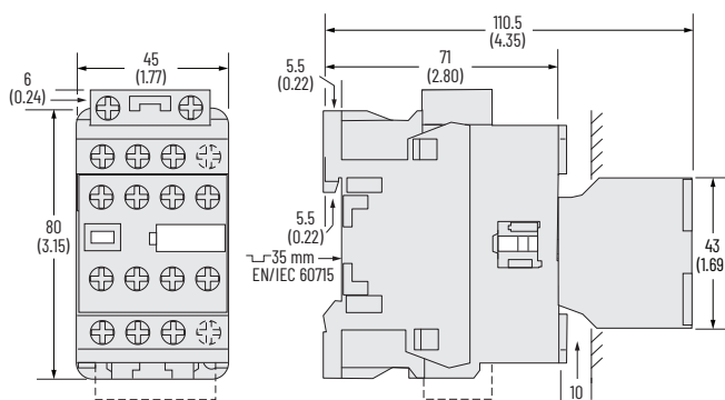
Figure 39 - 100-E09...100-E16 Contactors with Low-consumption Coils and Front-mounted Auxiliary Contact
