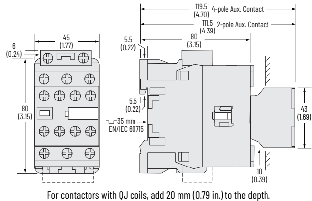
Figure 52 - 100-E26...100-E38 4-Pole Contactors with Low-consumption Coils and Front-mounted Auxiliary Contact
