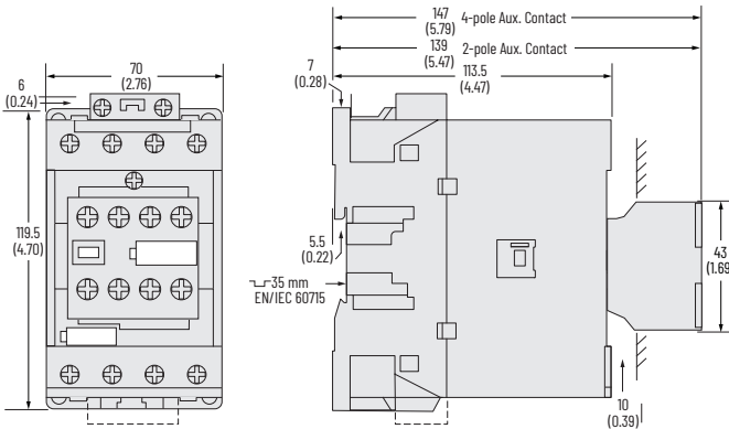
Figure 63 - 100-E40...100-E52 4-Pole Contactors with Front-mounted Auxiliary Contact
